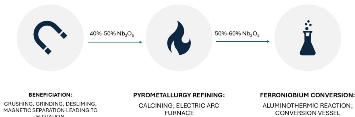
Figure 1 – simplified process flowsheet for niobium production from Araxa-style pyrochlore with typical grades achieved
