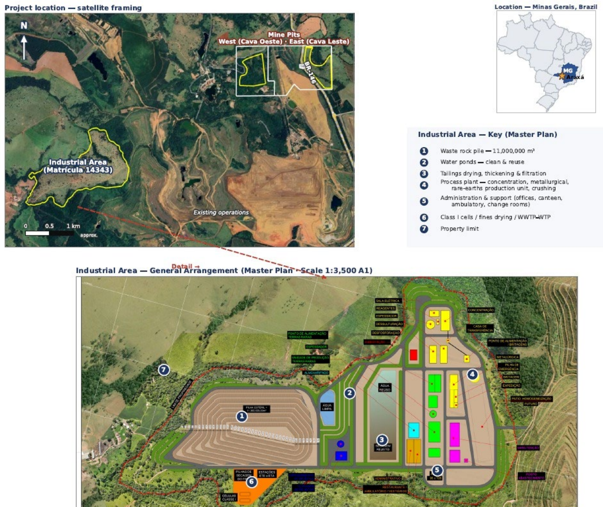
Figure 6 – schematic diagram showing the areas assessed for the potential mining operation and industrial complex at Araxá
