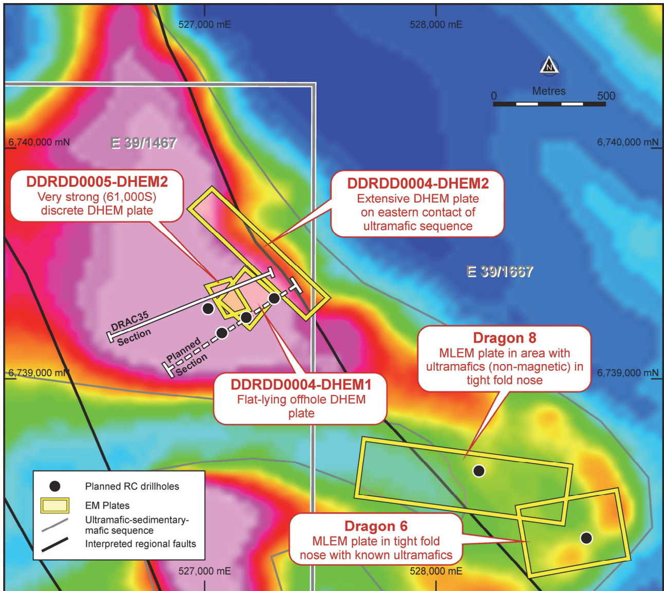
Figure 1 – a plan view of Desert Dragon Central with EM plates and planned holes against TMI magnetics. Drilling will now focus on testing the DHEM conductors.
