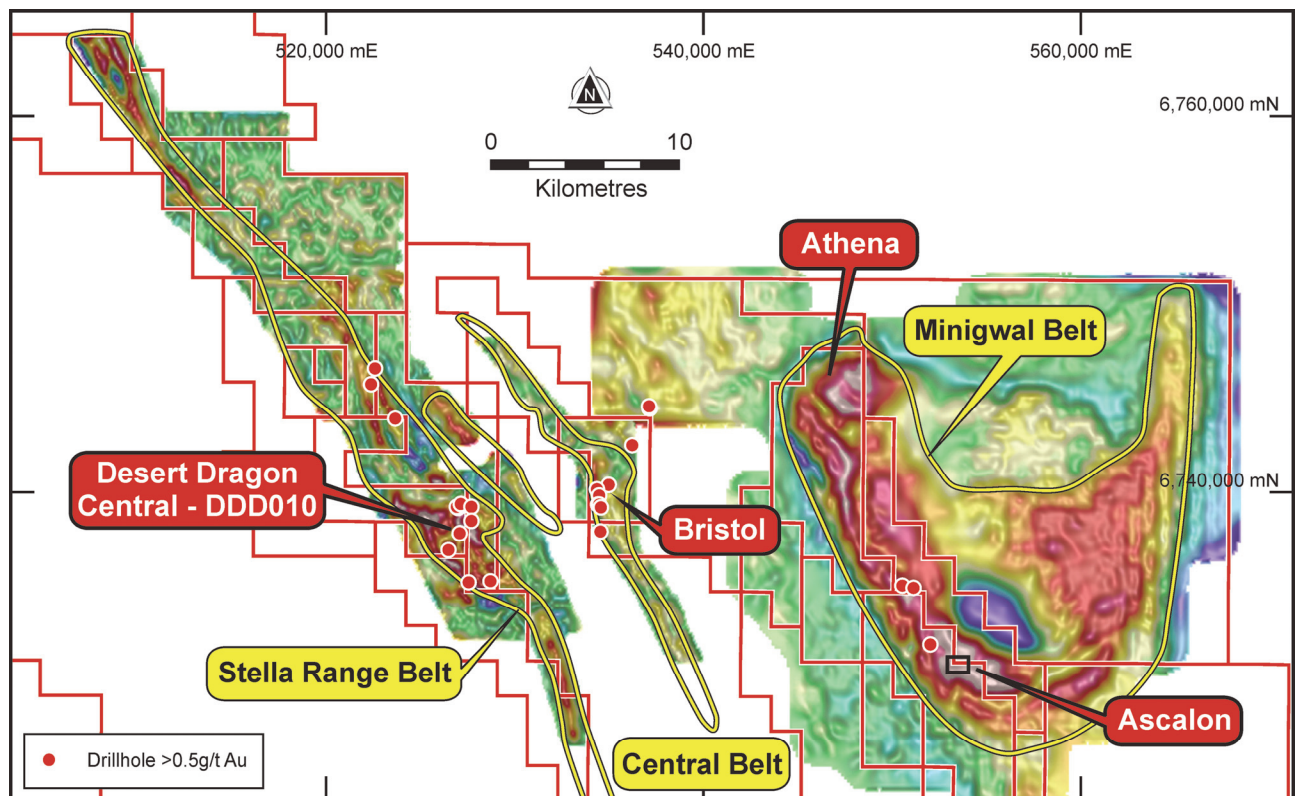
Figure 1 – the East Laverton tenements against FVD Bouguer gravity data with major gold targets highlighted. The gravity data has mapped the thick greenstones and complex structure at Athena. The greenstones have a variable strike, shifting from a northwest to a northerly and then to north-easterly orientation.
