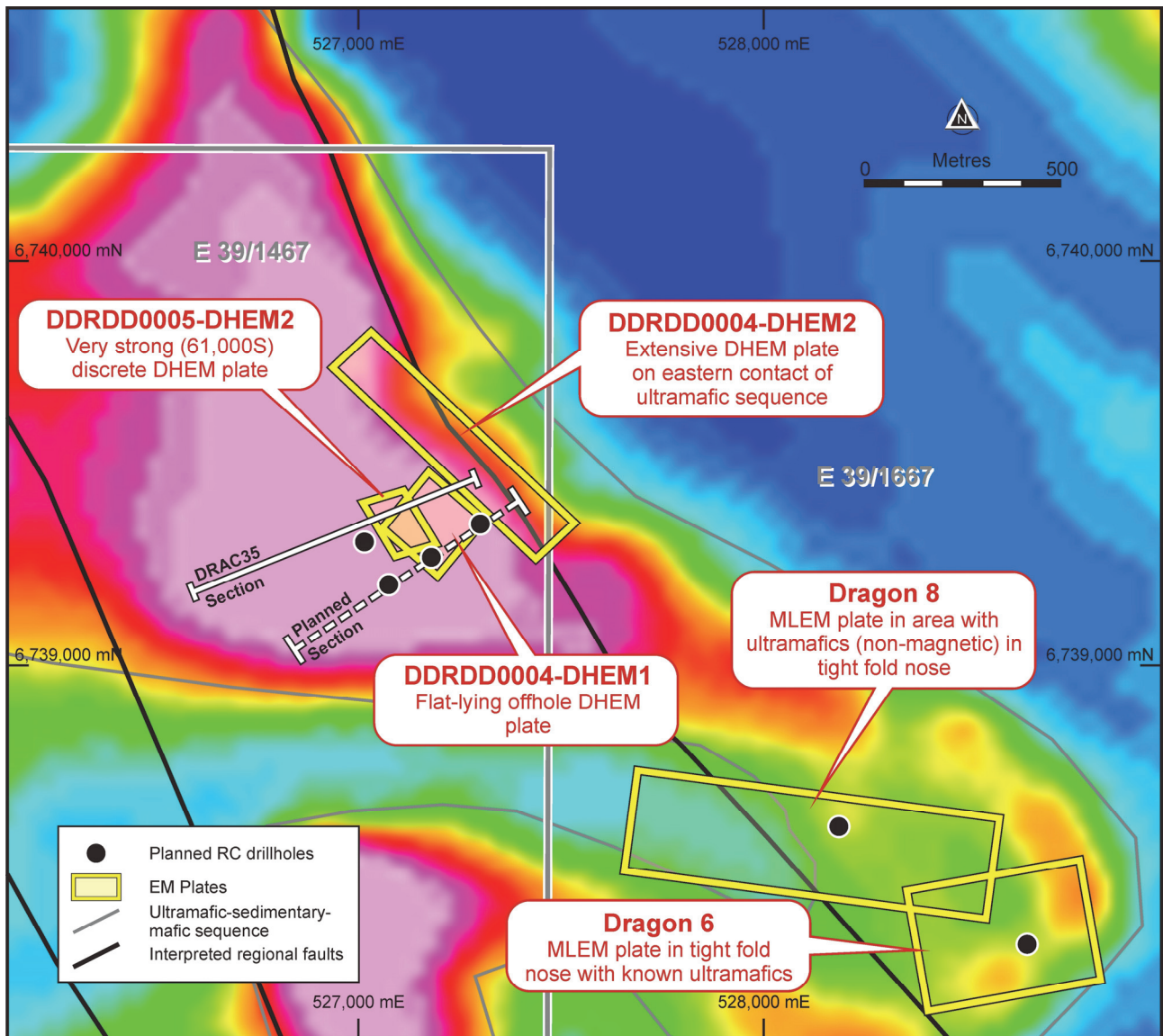
Figure 1 – a plan view of Desert Dragon Central with EM plates and planned holes against TMI magnetics. Dragon 6 and Dragon 8 are the first targets to be tested.
