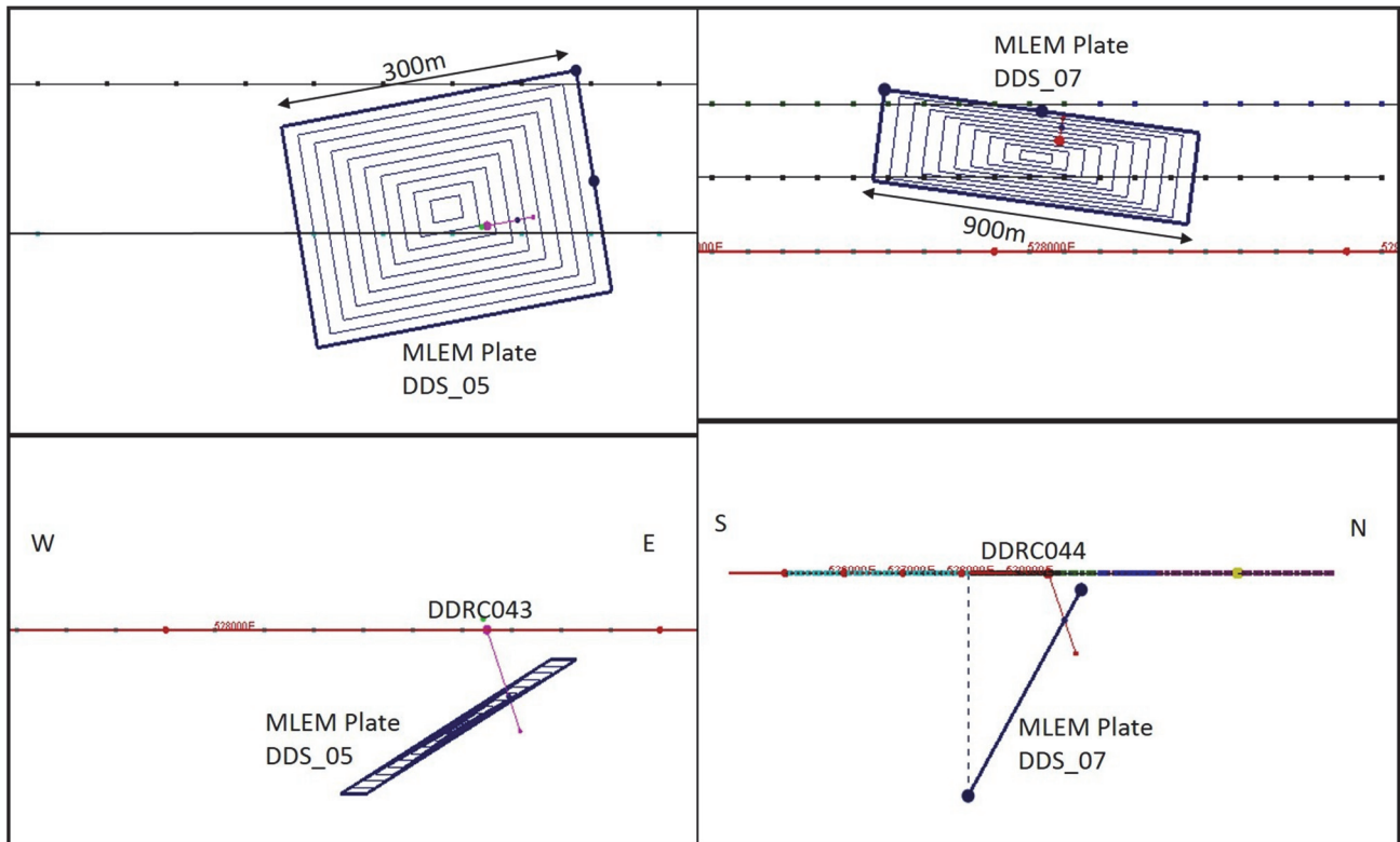
Figure 2 – plan view and cross section of drill holes to test Dragon 6 : MLEM Plate DDS_05 (left) and Dragon 8 : MLEM Plate DDS_07 (right)
